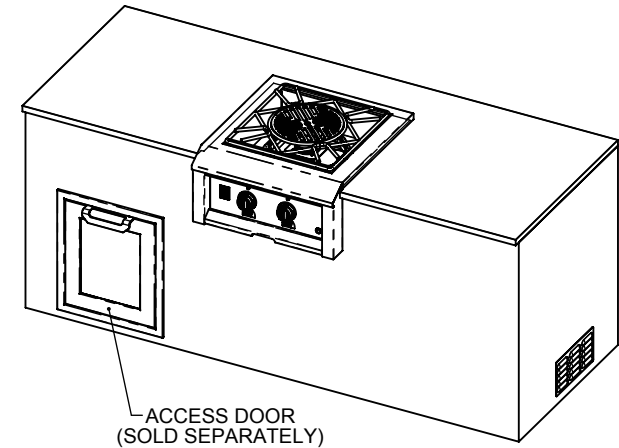
TYPICAL ISLAND COUNTERTOP INSTALLATION
